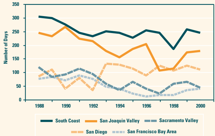
Calculated Days Over the State 24 hr PM10 Standard (50 µg/m³)
