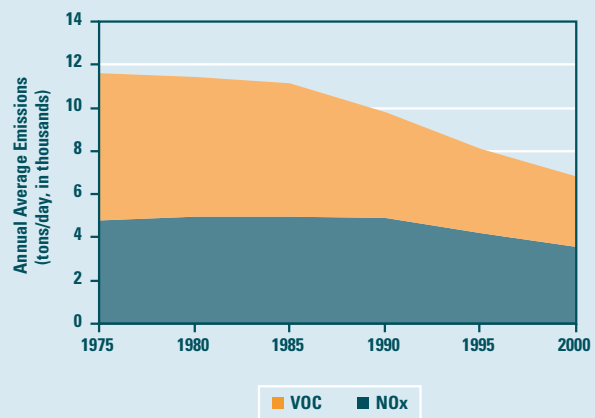
Volatile Organic Compound (VOC) and Nitrogen Oxide (NOx) Emission Trends
